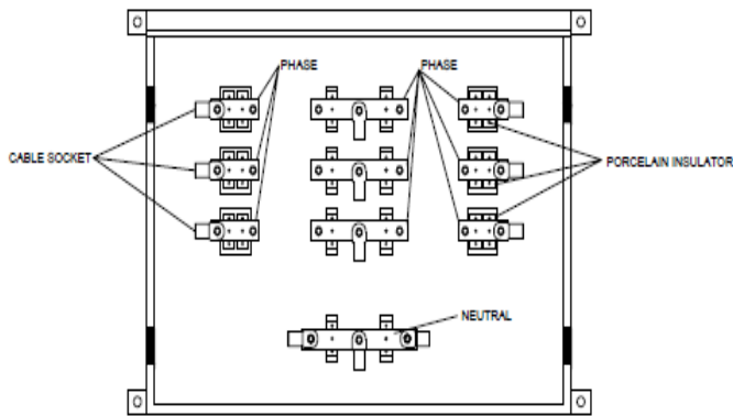
FRONT VIEW WITHOUT DOOR
