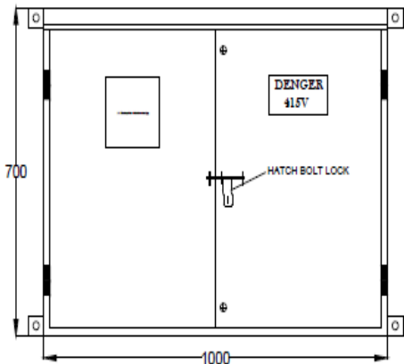
FRONT VIEW WITH DOOR
