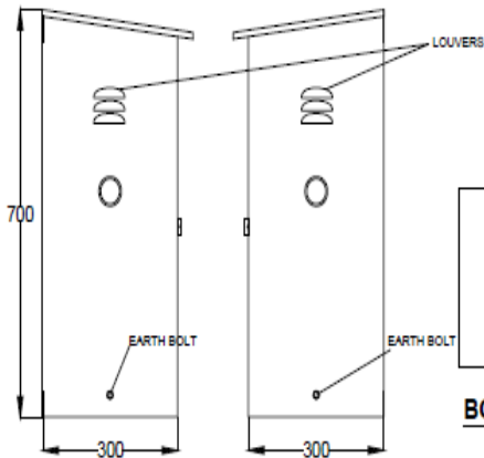
L.H.S VIEW
